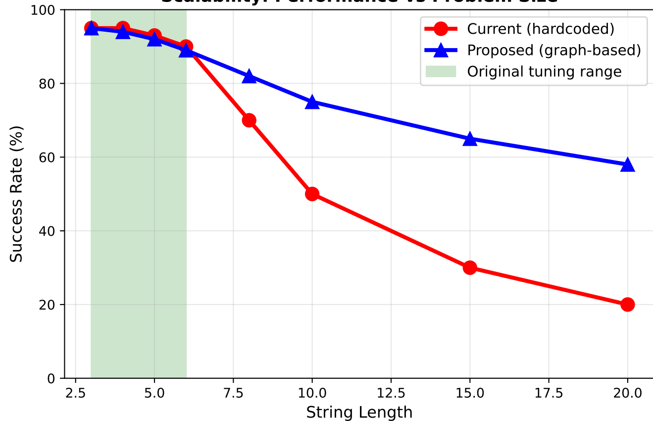
Scalability: Performance vs Problem Size
