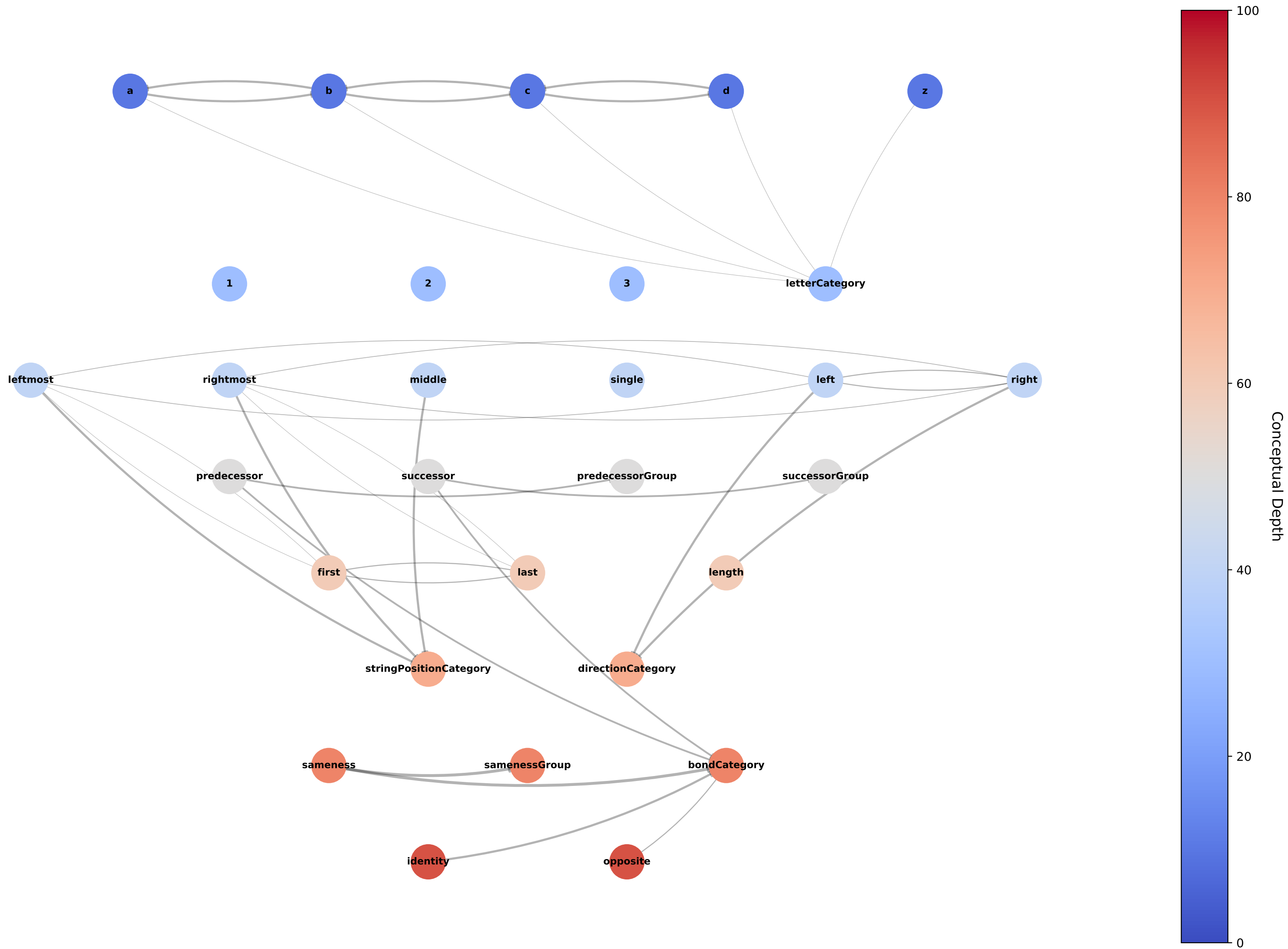
Slipnet Graph Structure Color gradient: Blue (concrete/shallow) → Red (abstract/deep) Edge thickness: Link strength (inverse of link length)
