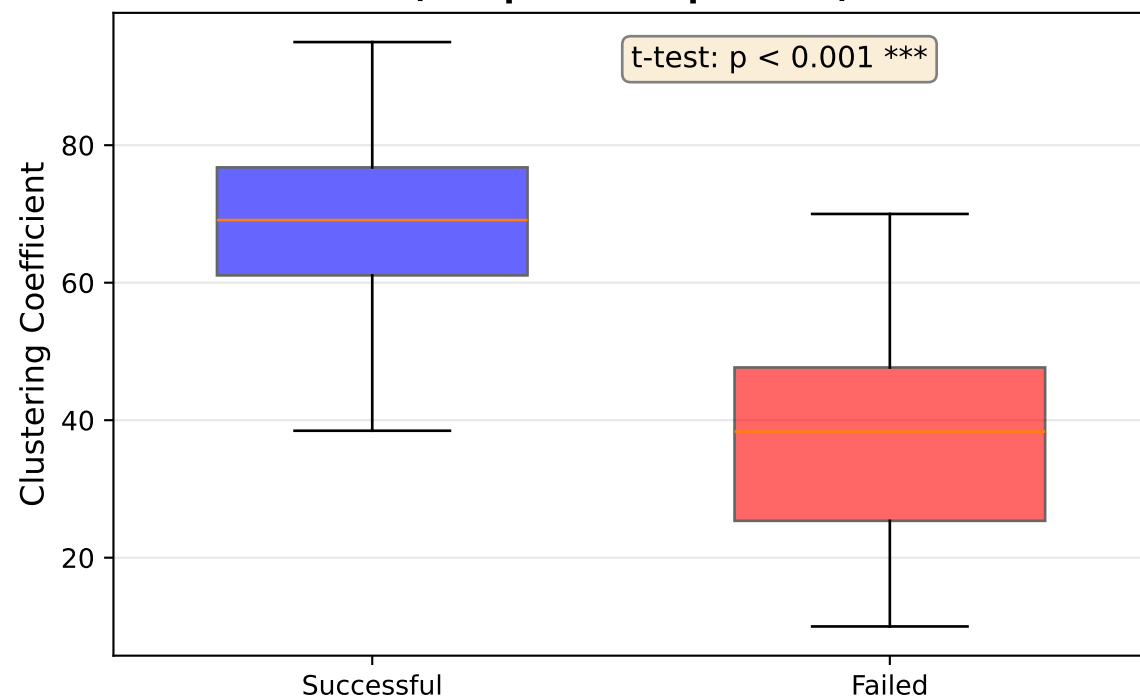
Statistical Comparison (Box plot with quartiles)
