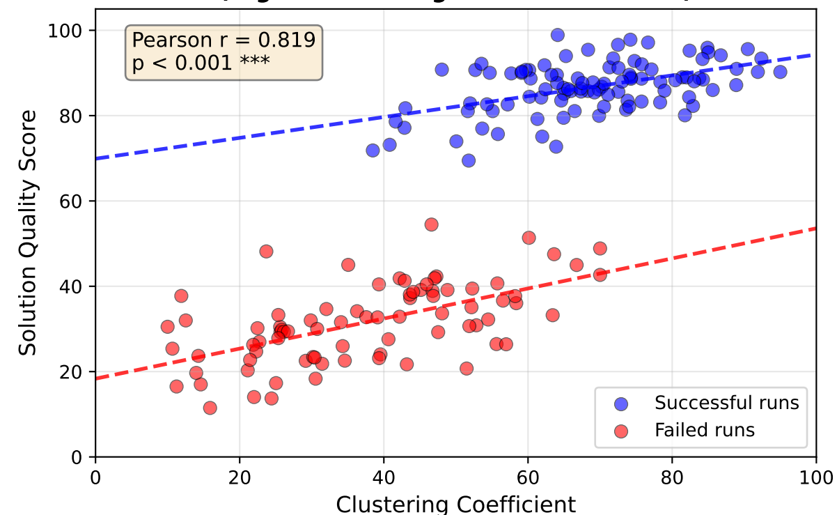
Correlation: Clustering vs Solution Quality (Higher clustering → better solutions)
